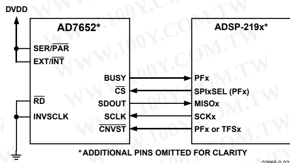
Figure 37. Interfacing the AD7652 to an SPI Interface
