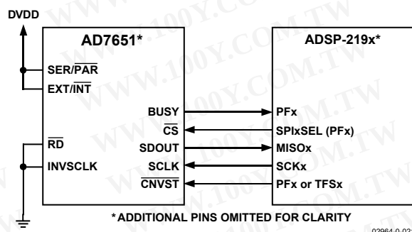
Figure 37. Interfacing the AD7651 to an SPI Interface
