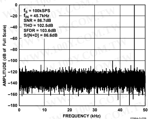
Figure 7. FFT Plot
