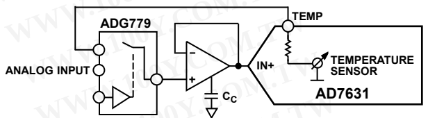
Figure 32. Use of the Temperature Sensor
