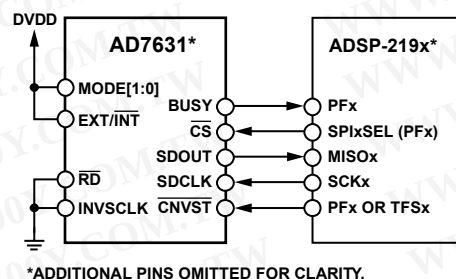
Figure 48. Interfacing the AD7631 to SPI Interface
