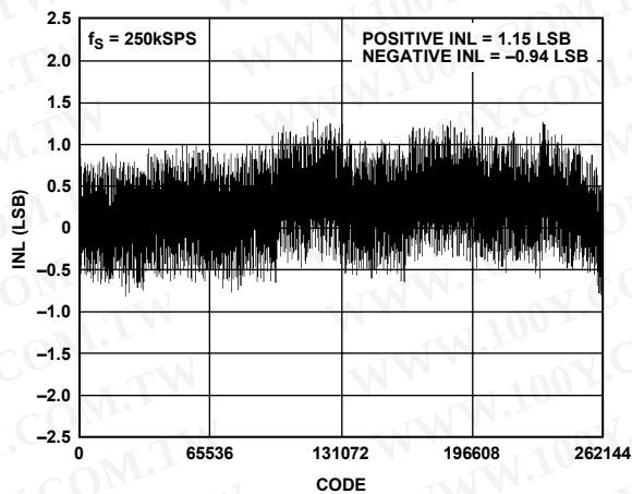
Figure 5. Integral Nonlinearity vs. Code, Bipolar 10 V Range
