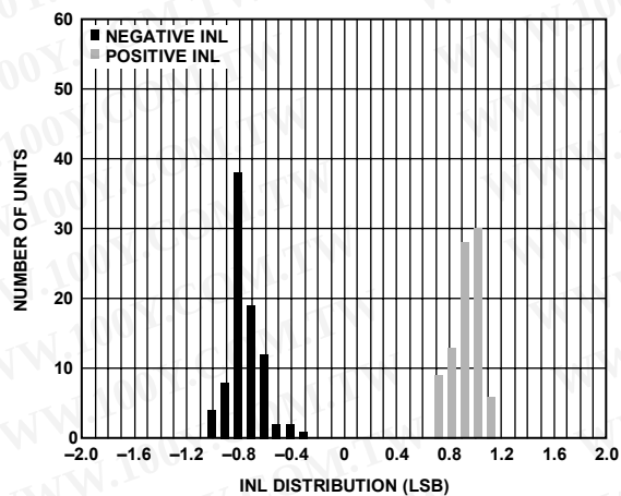
Figure 6. Integral Nonlinearity Distribution, Unipolar 10 V Range (86 Devices)
