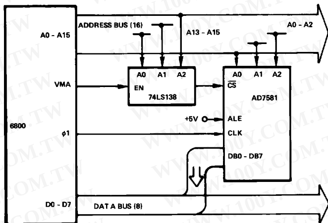
Figure 10. AD7581/6800 Interface
