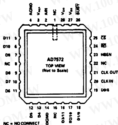
LCCC
