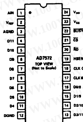
DIP
