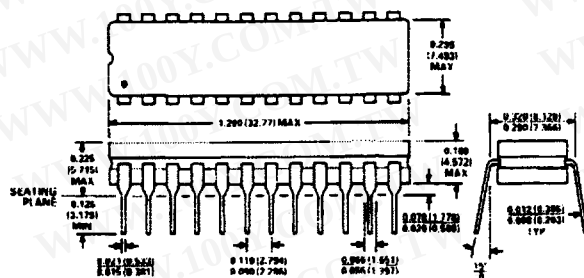
24-Pin Cerdip (Suffix Q)
