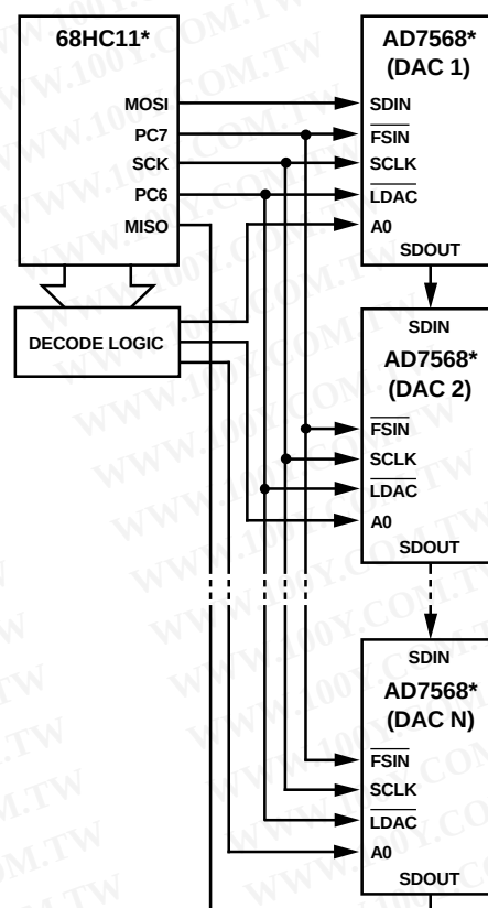
Figure 25. Multi-DAC System
