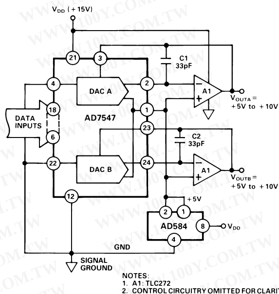
Figure 7. AD7547 Single Supply Operation
