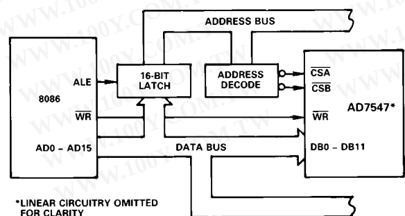
Figure 12. AD7547 - 8086 Interface
