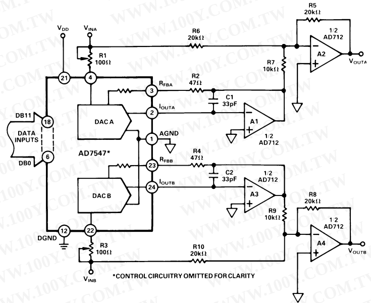
Figure 5. Bipolar Operation (Offset Binary Coding)
