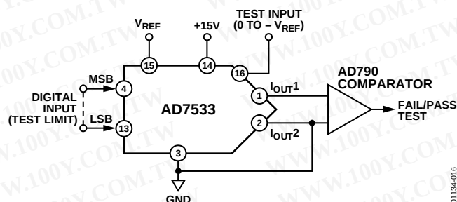
Figure 17. Digitally Programmable Limit Detector
