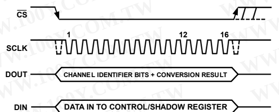
Figure 22. Normal Mode Operation
