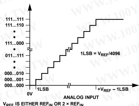
Figure 18. Straight Binary Transfer Characteristic
