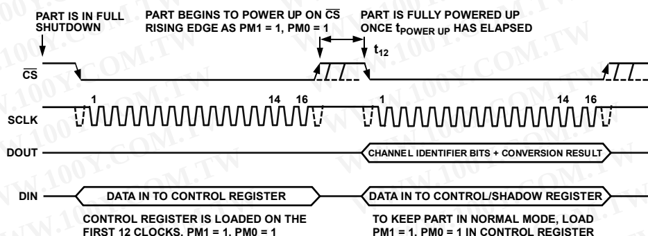
Figure 23. Full Shutdown Mode Operation
