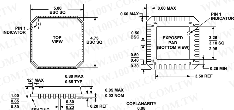
Figure 34. 32-Lead Lead Frame Chip Scale Package [LFCSQ_VQ] 5 mm × 5 mm Body, Very Thin Quad (CP-32-2)
