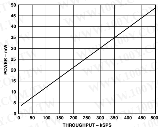
Figure 10. NAP Mode, Power vs. Throughput
