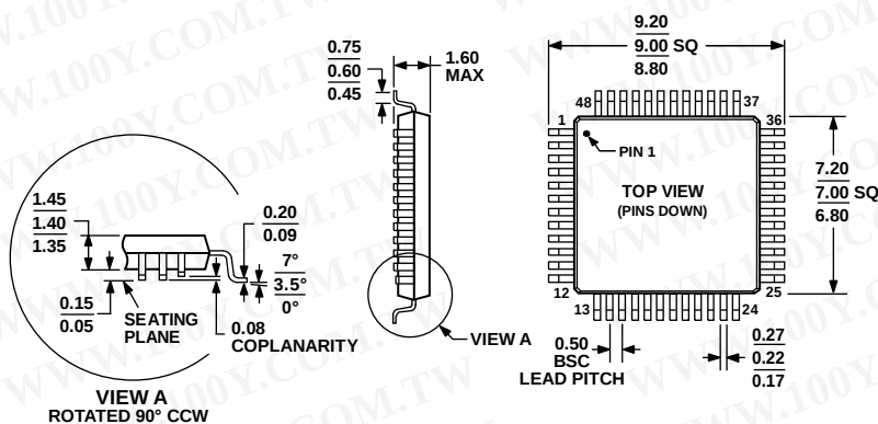
Figure 1. 48-Lead Low Profile Quad Flatpack [LQFP] 7 mm x 7 mm, Very Thin Quad (ST-48)
