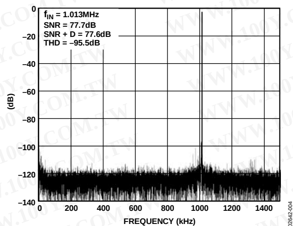
Figure 4. 64 k FFT Plot with 1 MHz Input Tone
