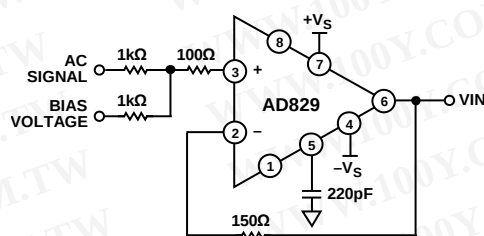
Figure 14. Analog Input Circuit Used for 10 kHz Input Tone
