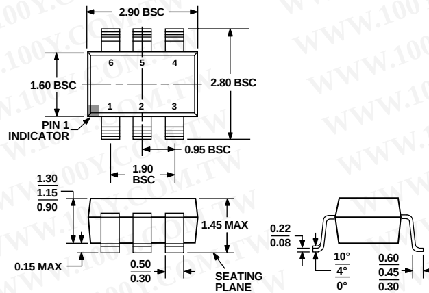
Figure 35. 6-Lead Small Outline Transistor Package [SOT-23] (RJ-6)
