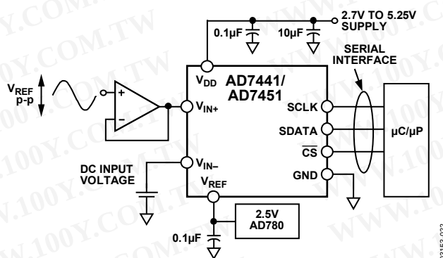
Figure 22. Typical Connection Diagram
