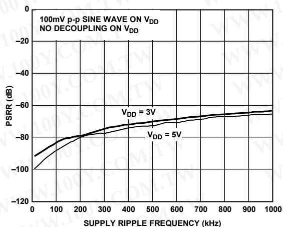
Figure 8. PSRR vs. Supply Ripple Frequency Without Supply Decoupling
