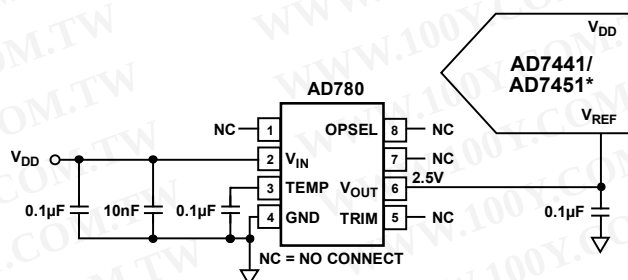
Figure 27. Typical V_{REF} Connection Diagram for V_{DD} = 5 V
