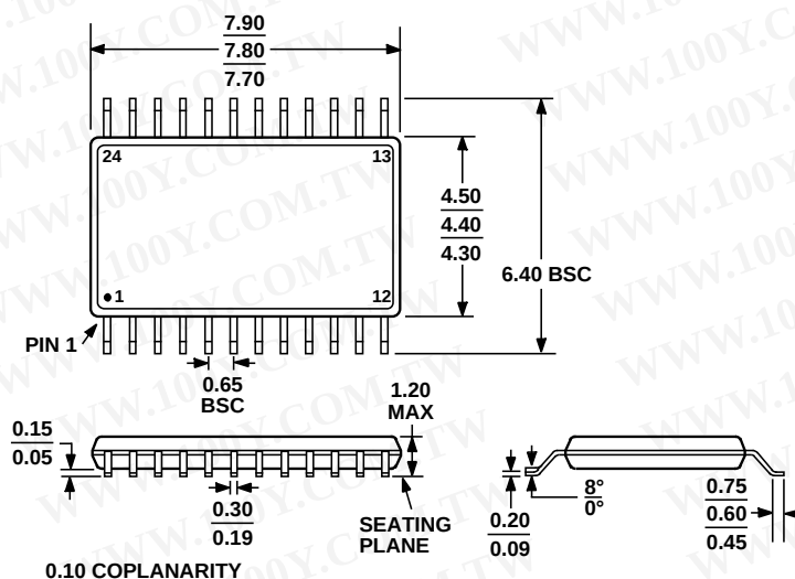
Figure 33. 24-Lead Thin Shrink Small Outline Package [TSSOP]
