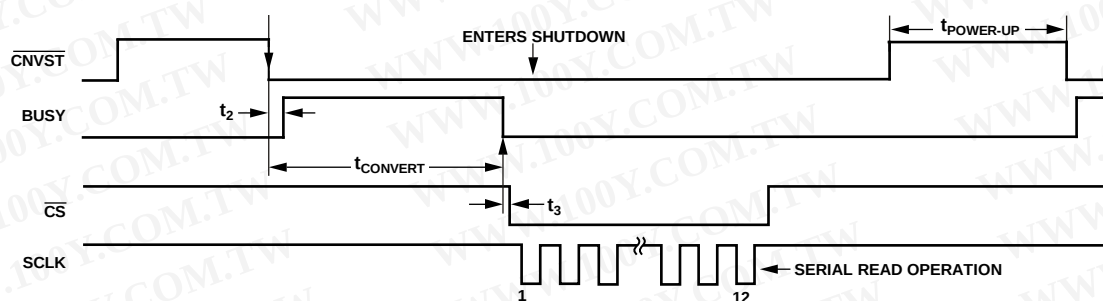
Figure 24. Autoshtutdown Mode for the AD7366
