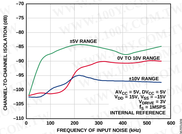
Figure 9. Channel-to-Channel Isolation
