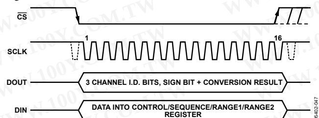
Figure 52. Normal Mode
