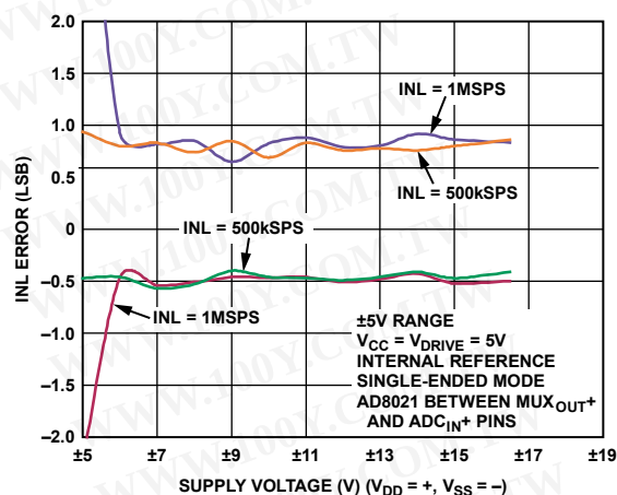
Figure 19. INL Error vs. Supply Voltage at 500 kSPS and 1 MSPS
