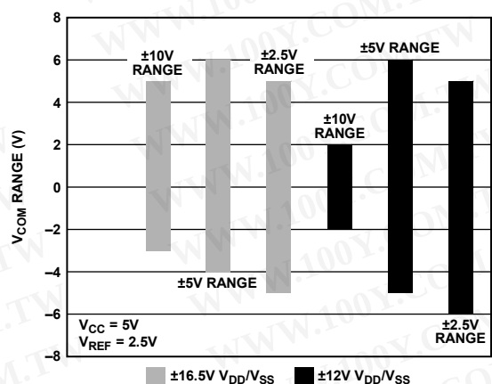
Figure 41. Common-Mode Range for V_{CC} = 5V and REF_{IN}/REF_{OUT} = 2.5V
