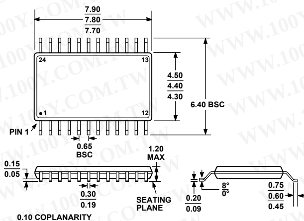
Figure 61. 24-Lead Thin Shrink Small Outline Package [TSSOP]
