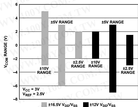
Figure 40. Common-Mode Range for V_{CC} = 3V and REF_{IN}/REF_{OUT} = 2.5V
