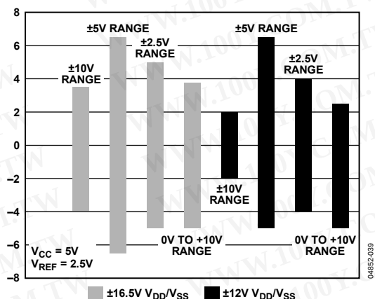
Figure 40. Pseudo Differential Input Range with V_{CC} = 5V
