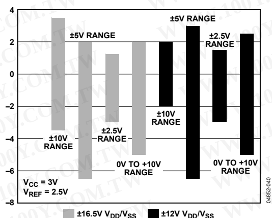
Figure 41. Pseudo Differential Input Range with V_{CC} = 3V
