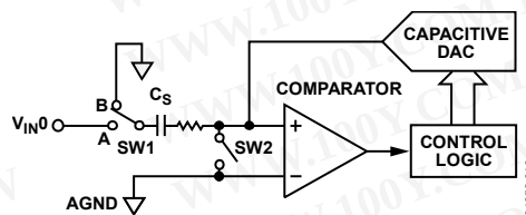
Figure 24. ADC Configuration During Conversion Phase, Single-Ended Mode
