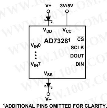
1ADDITIONAL PINS OMITTED FOR CLARITY. Figure 56. Schottky Diode Connection
