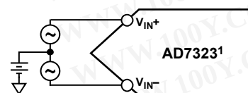
Figure 34. True Differential Inputs
