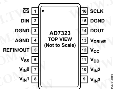
Figure 3. Pin Configuration
