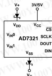
Figure 53. Schottky Diode Connection
