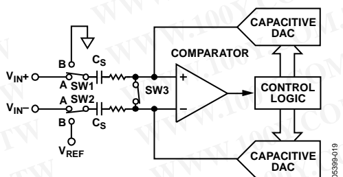
Figure 25. ADC Differential Configuration During Acquisition Phase
