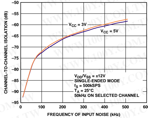
Figure 14. Channel-to-Channel Isolation
