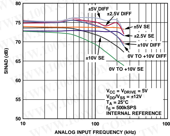
Figure 13. SINAD vs. Analog Input Frequency for Single-Ended (SE) and True Differential Mode (Diff) at 5V V_{CC}
