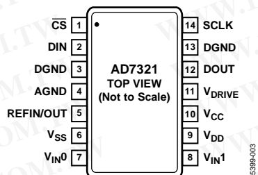
Figure 3. Pin Configuration
