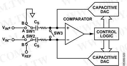
Figure 26. ADC Differential Configuration During Conversion Phase
