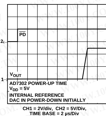
Figure 10. Exiting Power-Down (Full Power-Down)
