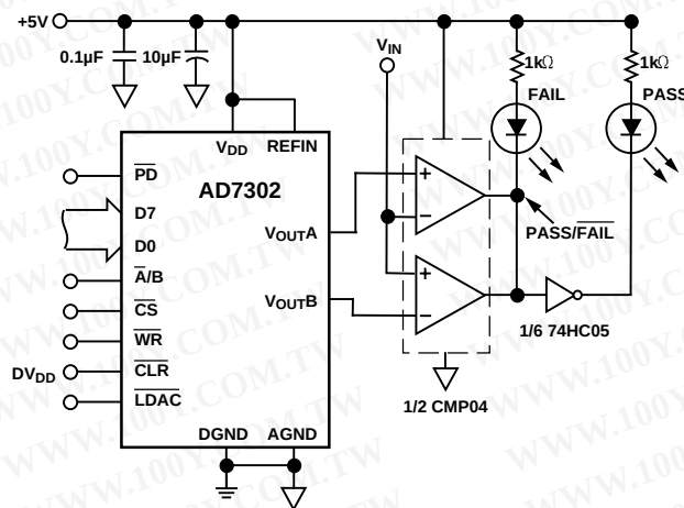
Figure 34. Programmable Window Detector
