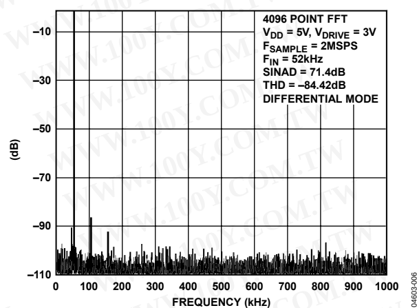
Figure 7. FFT
