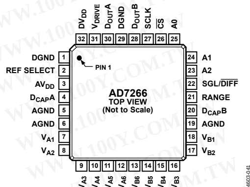
Figure 3. Pin Configuration (SU-32-2)
