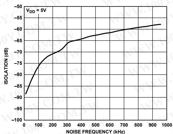
Figure 5. Channel-to-Channel Isolation
