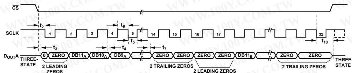
Figure 42. Reading Data from Both ADCs on One D_{OUT} Line with 32 SCLKs
