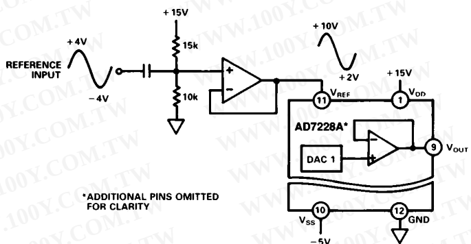
Figure 9. Applying a AC Signal to the AD7228A
