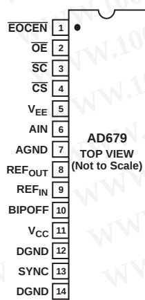
DIP Package
