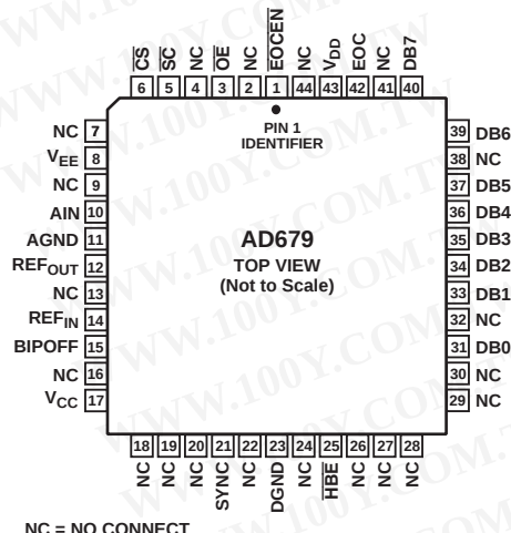
JLCC Package
