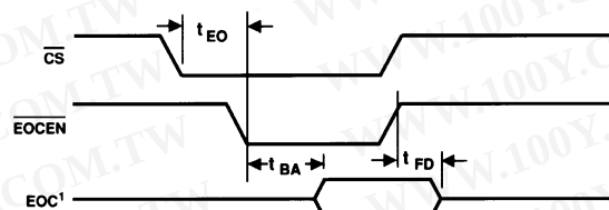
Figure 2. EOC Timing
