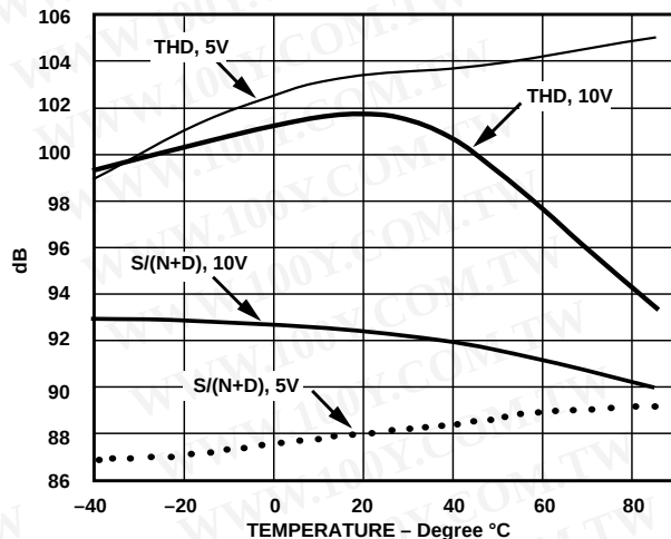
Figure 18. AC Performance Using Minimum Clock Period vs. Temperature ( t_{CLK} = 480 \text{ ns} ), 5 V and 10 V Reference
