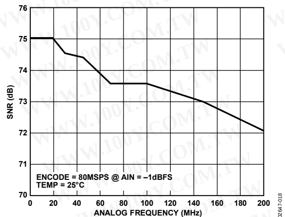
Figure 12. Signal-to-Noise Ratio (SNR) vs. Analog Frequency (IF)
