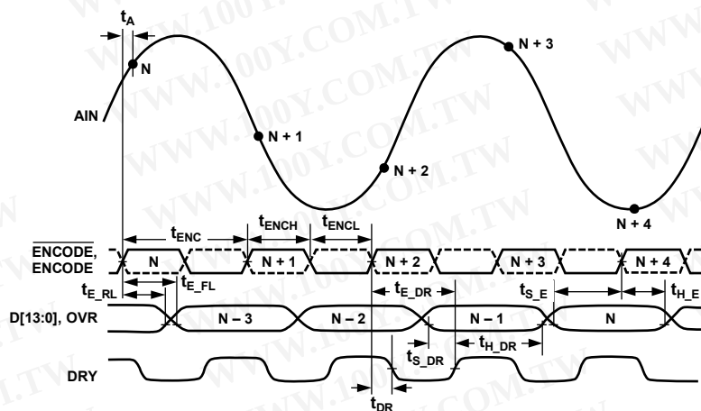
Figure 2. Timing Diagram
