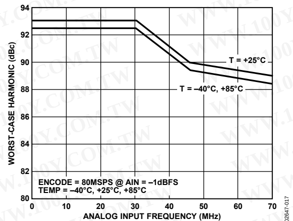
Figure 11. Worst-Case Harmonics vs. Analog Input Frequency
