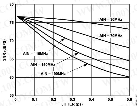
Figure 42. SNR vs. Jitter
