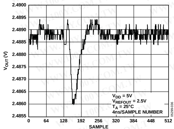
Figure 36. DAC-to-DAC Crosstalk
