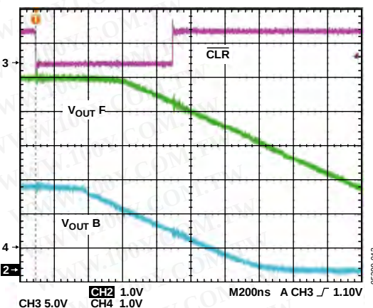
Figure 43. Hardware \overline{\text{CLR}}
