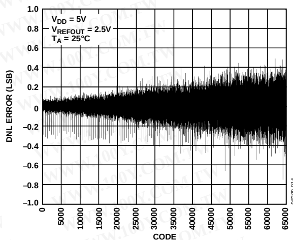
Figure 8. DNL 16-Bit DAC, 2.5 V Internal Reference
