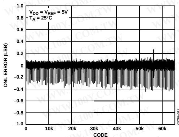
Figure 6. DNL—16-Bit DAC
