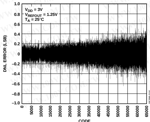
Figure 10. DNL—16-Bit DAC, 1.25 V Internal Reference
