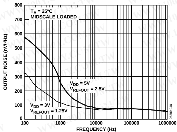
Figure 40. Noise Spectral Density, Internal Reference
