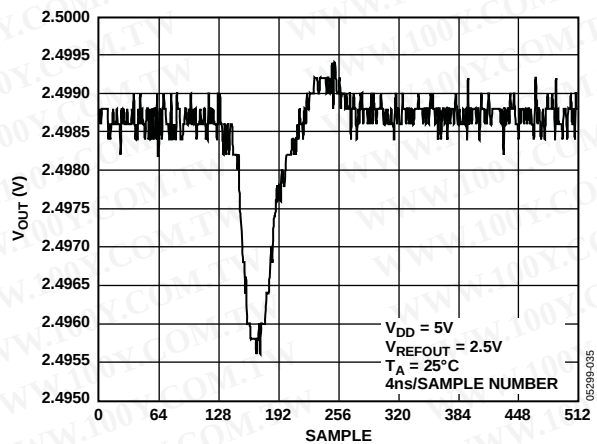
Figure 35. Analog Crosstalk
