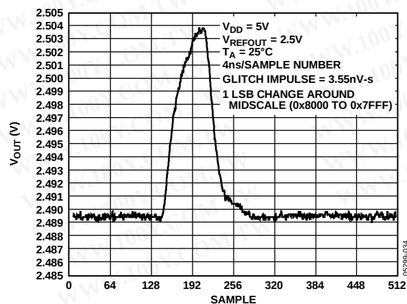
Figure 34. Digital-to-Analog Glitch Impulse (Negative)
