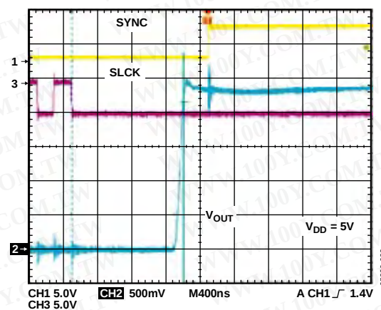
Figure 33. Exiting Power-Down to Midscale
