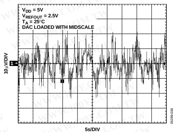
Figure 38. 0.1 Hz to 10 Hz Output Noise Plot, Internal Reference
