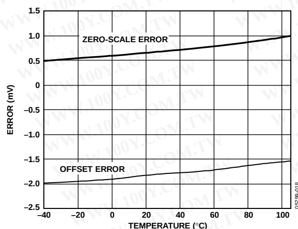
Figure 18. Zero-Scale Error and Offset Error vs. Temperature
