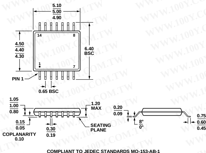
Figure 51. 14-Lead Thin Shrink Small Outline Package [TSSOP] (RU-14) Dimensions shown in millimeters
