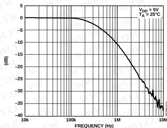
Figure 44. Multiplying Bandwidth
