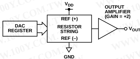
Figure 27. DAC Architecture
