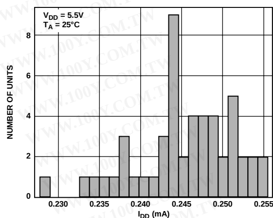
Figure 13. I_{DD} Histogram with V_{DD} = 5.5\text{ V}
