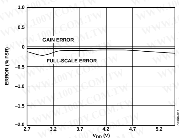
Figure 11. Gain Error and Full-Scale Error vs. Supply
