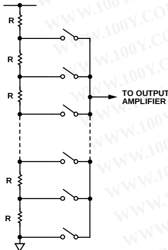
Figure 28. Resistor String
