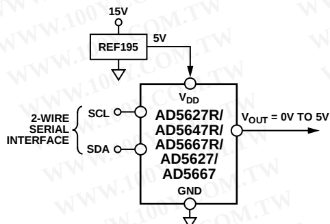
Figure 67. REF195 as Power Supply to the AD56x7R/AD56x7
