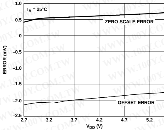
Figure 30. Zero-Scale Error and Offset Error vs. Supply
