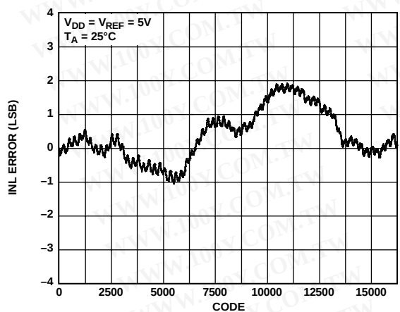
Figure 7. AD5647R INL, External Reference
