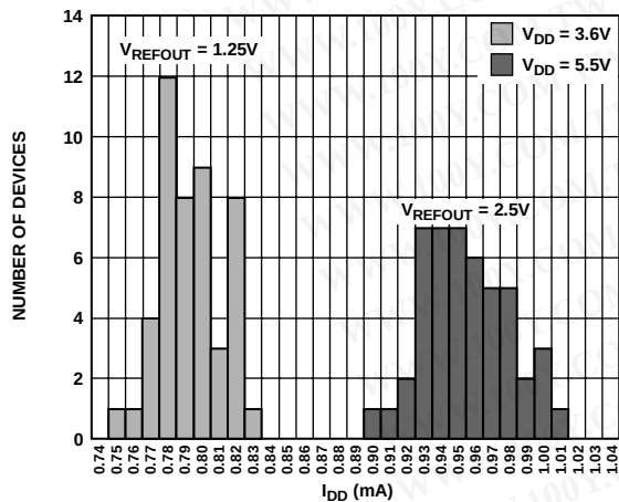
Figure 32. I_{DD} Histogram with Internal Reference
