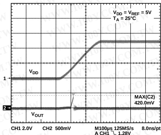
Figure 40. Power-On Reset to 0 V
