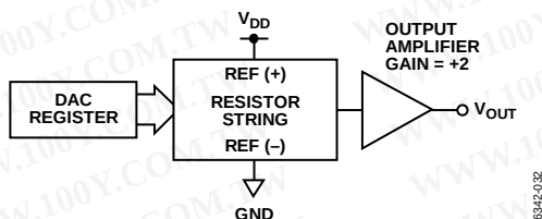
Figure 52. DAC Architecture
