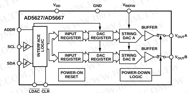
Figure 2. AD5627/AD5667
