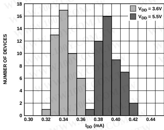
Figure 31. I_{DD} Histogram with External Reference
