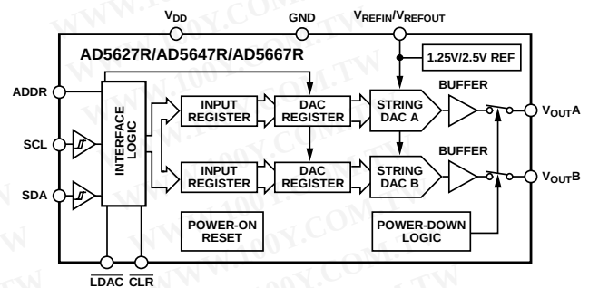
Figure 1. AD5627R/AD5647R/AD5667R
