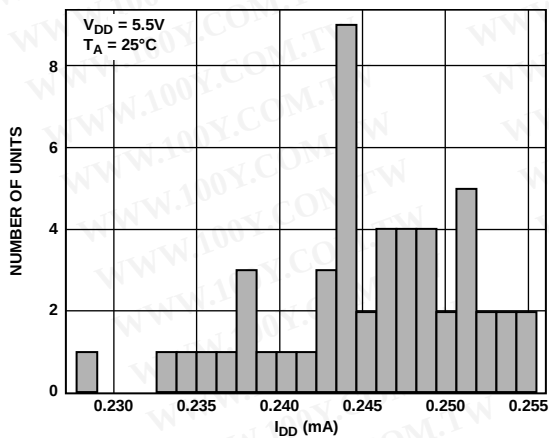
Figure 29. I_{DD} Histogram with External Reference
