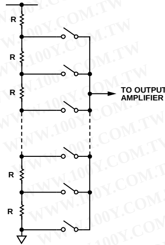
Figure 50. Resistor String
