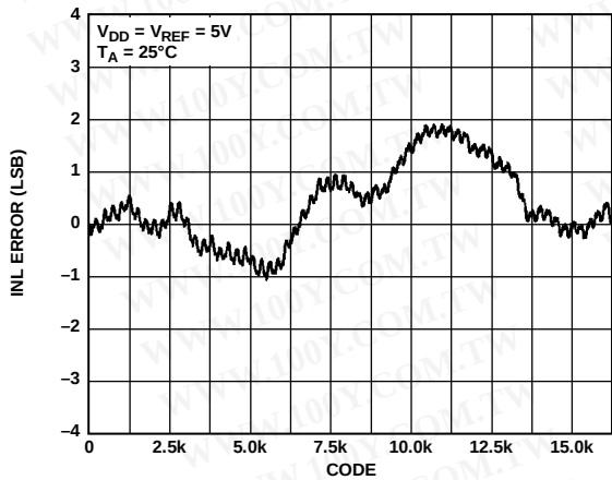
Figure 5. INL—AD5643R, External Reference
