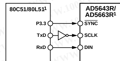
Figure 58. AD5623R/AD5643R/AD5663R to 80C51/80L51 Interface
