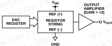
Figure 49. DAC Architecture
