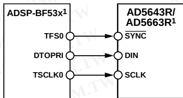
Figure 56. AD5623R/AD5643R/AD5663R to Blackfin ADSP-BF53X Interface
