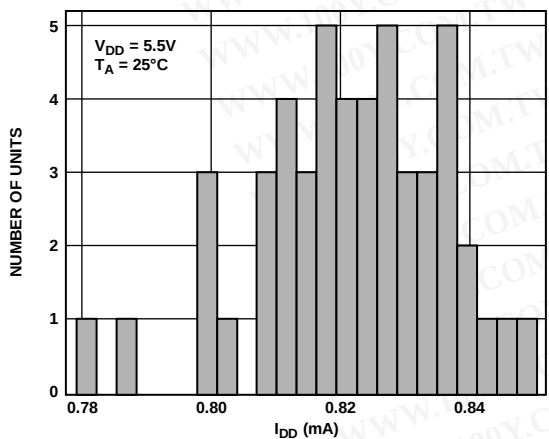
Figure 30. I_{DD} Histogram with Internal Reference
