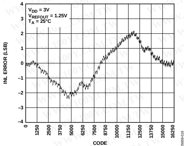
Figure 17. INL—AD5643R-3
