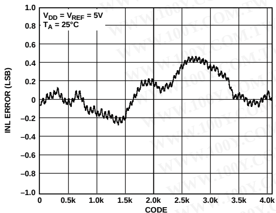
Figure 6. INL—AD5623R, External Reference
