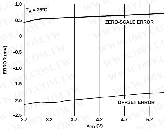
Figure 28. Zero-Scale Error and Offset Error vs. Supply
