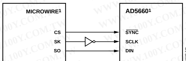
Figure 48. AD5660-to-MICROWIRE Interface
