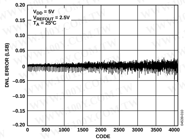
Figure 10. DNL—AD5620-2/AD5620-3
