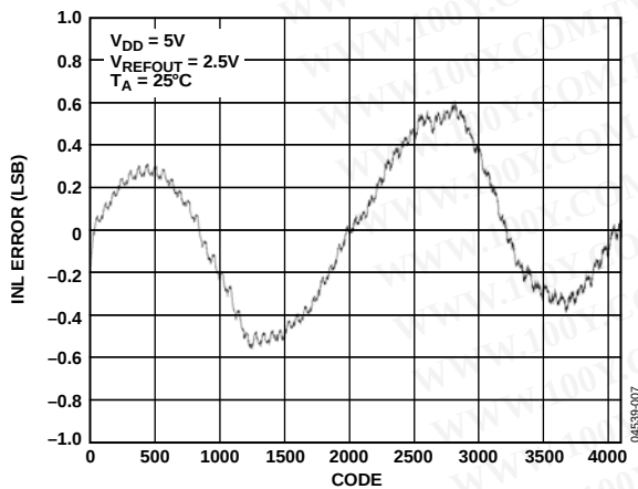
Figure 7. INL—AD5620-2/AD5620-3
