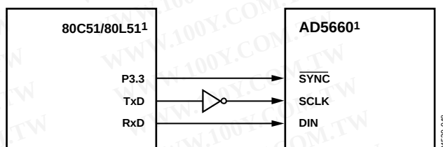
Figure 47. AD5660-to-80C51/80L51 Interface
