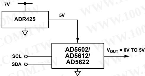
Figure 49. ADR425 as Power Supply
