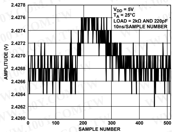
Figure 33. Digital Feedthrough
