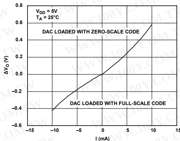
Figure 26. Sink and Source Capability
