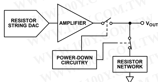
Figure 41. Output Stage During Power-Down
