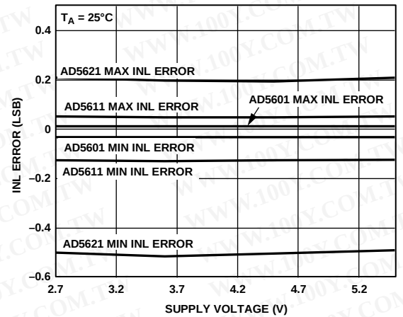
Figure 32. INL vs. Supply Voltage at 25°C
