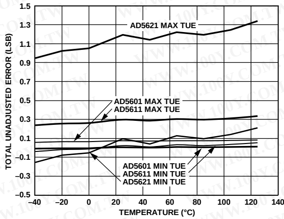
Figure 28. Total Unadjusted Error (TUE) vs. Temperature (5 V)
