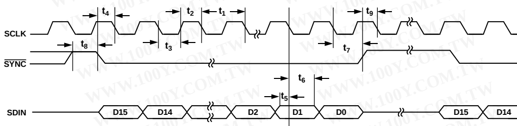
Figure 2. Timing Diagram
