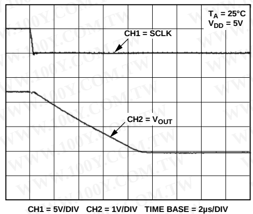
Figure 15. Half-Scale Settling Time
