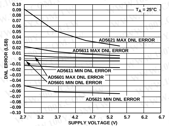
Figure 33. DNL vs. Supply Voltage at 25°C
