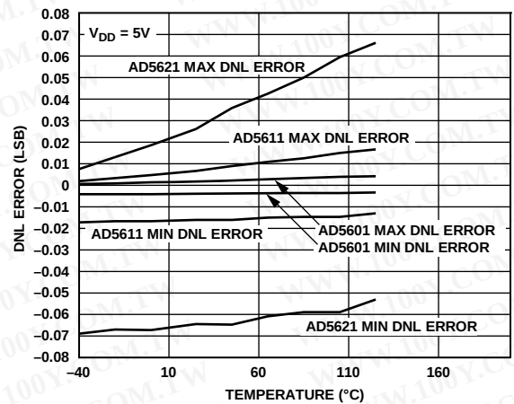
Figure 26. DNL vs. Temperature (5 V)
