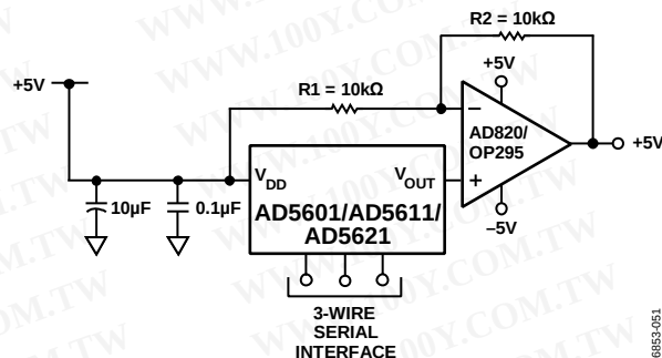
Figure 51. Bipolar Operation with the AD5601/AD5611/AD5621
