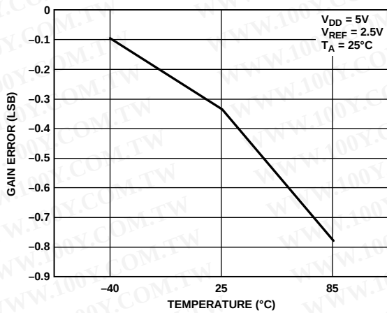
Figure 12. Gain Error vs. Temperature
