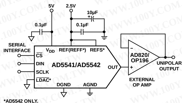
Figure 23. Unipolar Output
