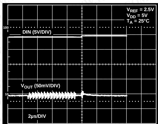
Figure 18. Digital Feedthrough
