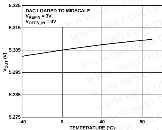
Figure 12. V_{OUT} vs. Temperature
