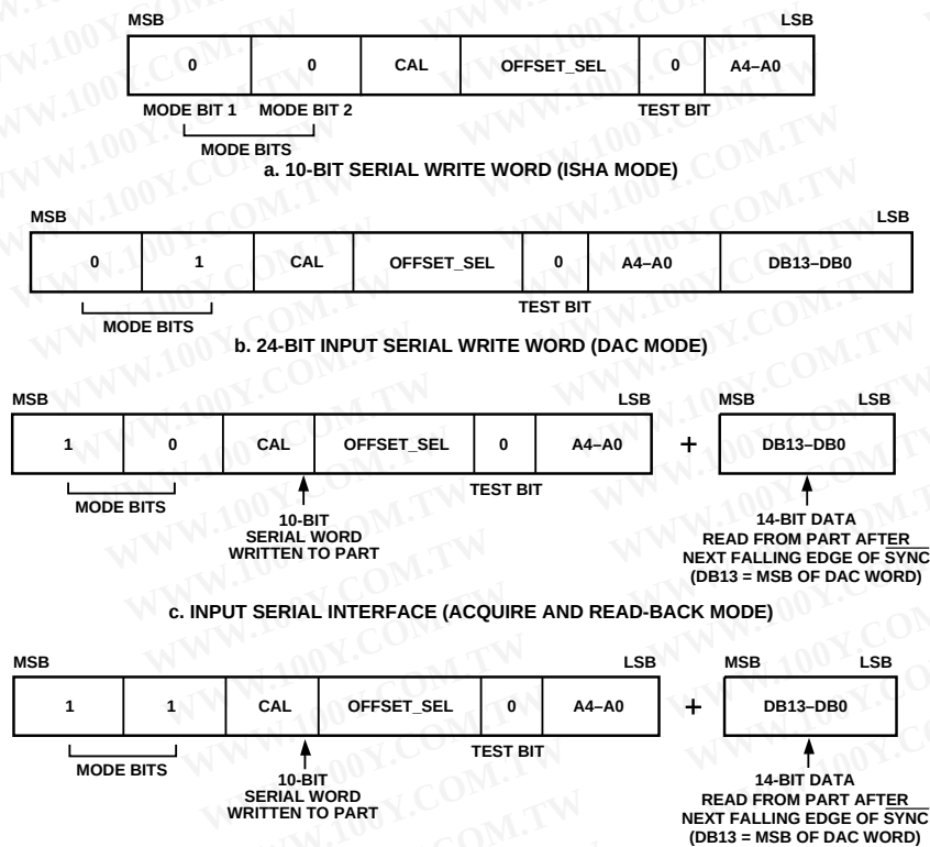
Figure 21. Serial Interface Formats
