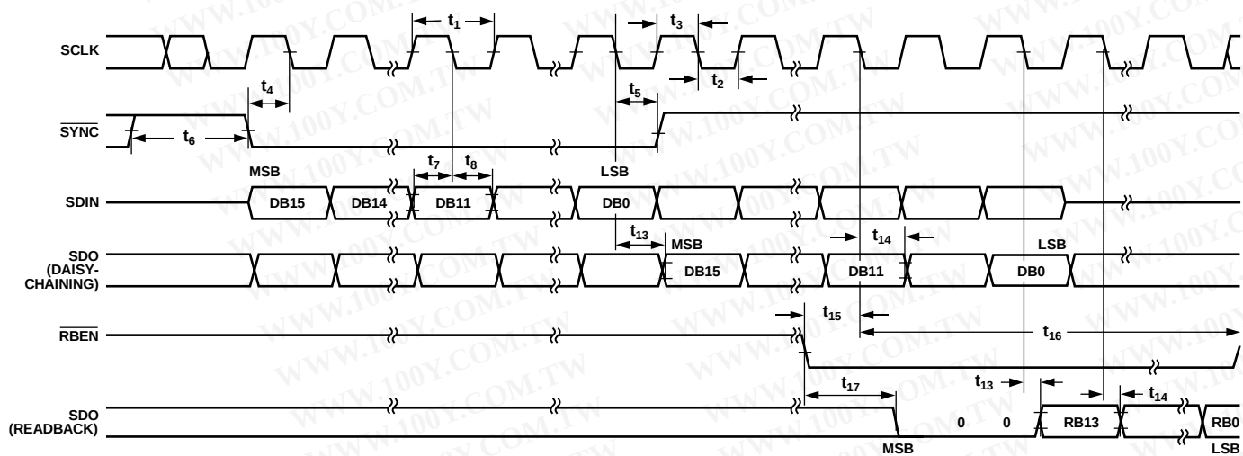
Figure 3. Timing Diagram for Daisy-Chaining and Readback Mode
