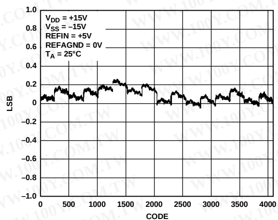
Figure 5. AD5530 Typical INL Plot
