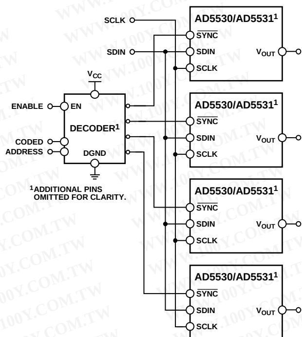
Figure 27. Addressing Multiple AD5530/AD5531s
