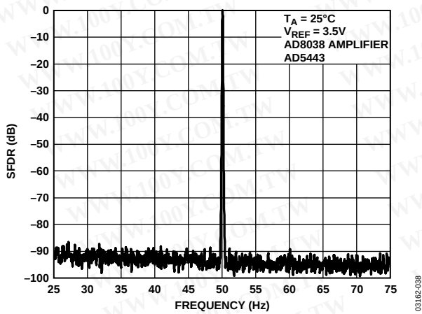
Figure 37. Narrowband (±50%) SFDR f_{OUT} = 50 kHz, Update = 1 MHz
