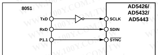
Figure 55. 80C51/80L51-to-AD5426/AD5432/AD5443 Interface
