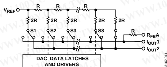
Figure 40. Simplified Ladder
