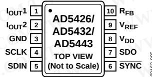
Figure 5. Pin Configuration
