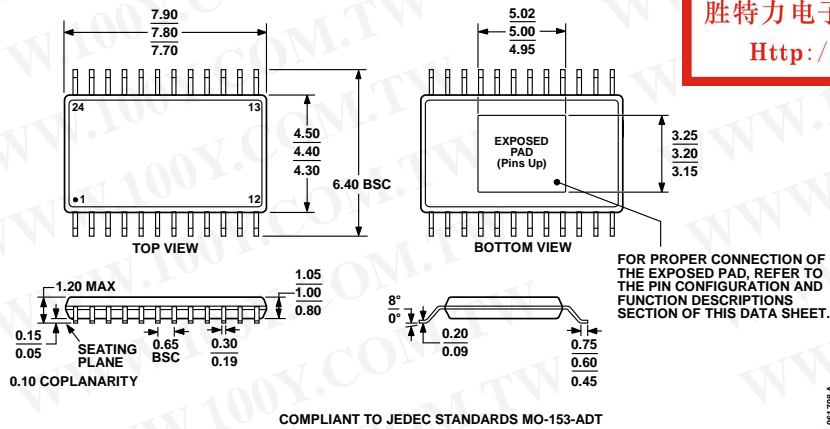
Figure 81. 24-Lead Thin Shrink Small Outline Package, Exposed Pad [TSSOP_EP] (RE-24) Dimensions shown in millimeters
