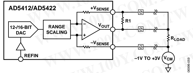
Figure 65. Voltage Output
