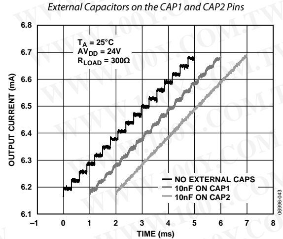
Figure 73. Smoothing Out the Steps Caused by the Digital Slew Rate Control Feature
