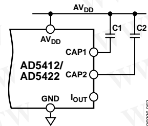
Figure 70. I_{\text{OUT}} Filtering Capacitors
