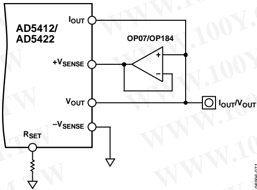
Figure 74. Isolated Interface
