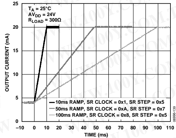
Figure 69. Output Current Slew Under Control of the Digital Slew Rate Control Feature
