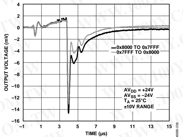
Figure 38. Digital-to-Analog Glitch
