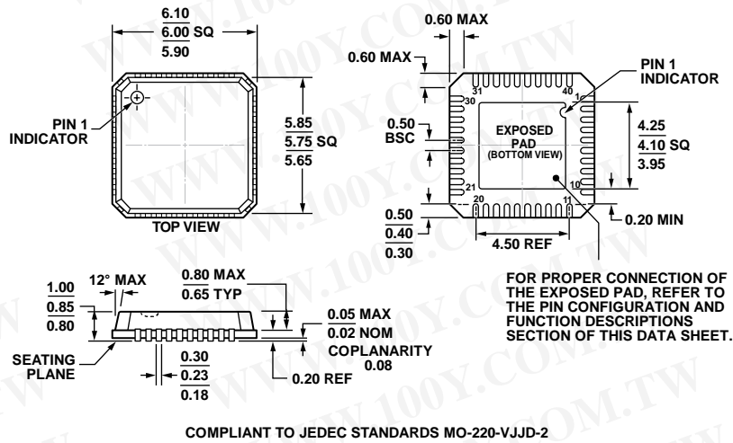
Figure 82. 40-Lead Lead Frame Chip Scale Package [LFCSP_VQ] 6 mm x 6 mm Body, Very Thin Quad (CP-40-1) Dimensions shown in millimeters
