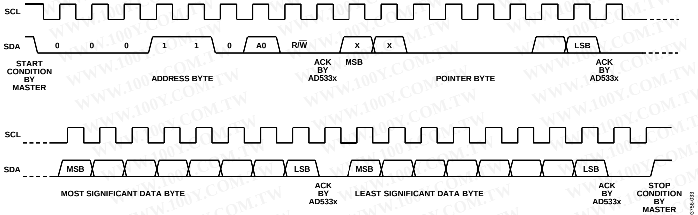
Figure 33. Write Sequence
