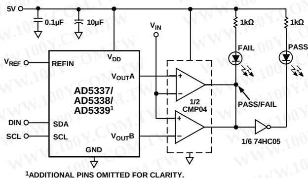
Figure 39. Window Detection
