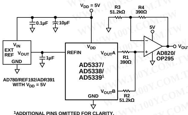
Figure 40. Coarse/Fine Adjustment
