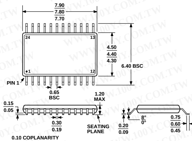
Figure 49. 24-Lead Thin Shrink Small Outline Package [TSSOP] (RU-24) Dimensions shown in millimeters
