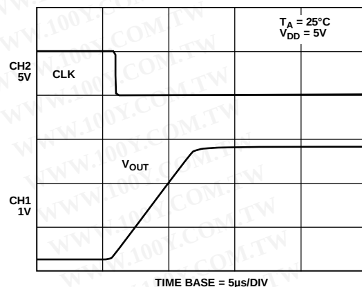
Figure 29. Half-Scale Settling (1/4 to 3/4 Scale Code Change)
