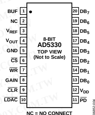
Figure 4. AD5330 Pin Configuration
