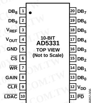
Figure 6. AD5331 Pin Configuration
