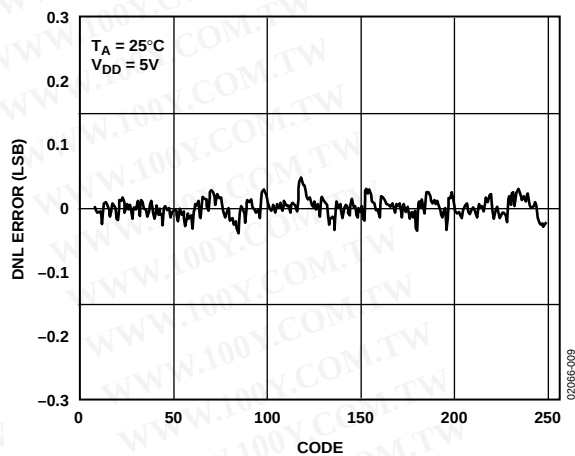
Figure 9. AD5306 DNL
