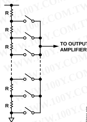
Figure 30. Resistor String
