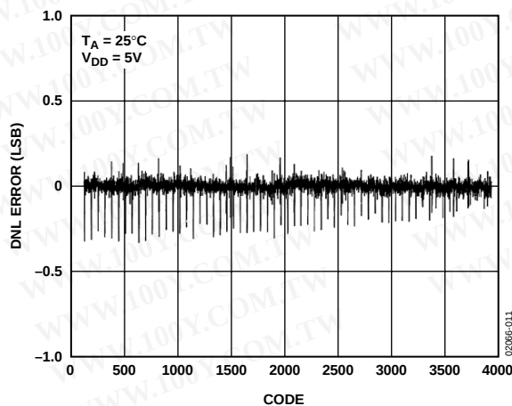
Figure 11. AD5326 DNL
