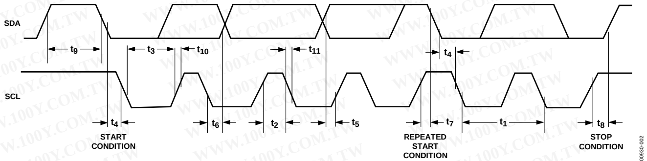
Figure 2. 2-Wire Serial Interface Timing Diagram
