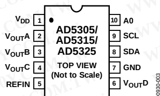
Figure 3. Pin Configuration
