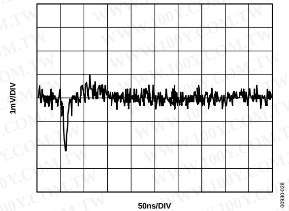
Figure 26. DAC-to-DAC Crosstalk
