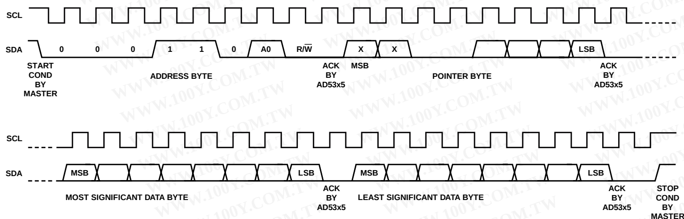
Figure 33. Write Sequence
