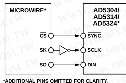
Figure 39. AD5304/AD5314/AD5324 to MICROWIRE Interface
