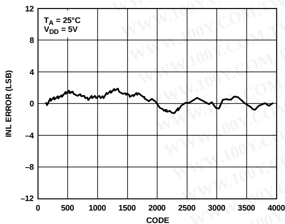
Figure 7. AD5324 Typical INL Plot
