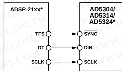
Figure 36. AD5304/AD5314/AD5324 to ADSP-21xx Interface
