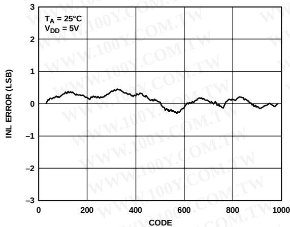
Figure 6. AD5314 Typical INL Plot
