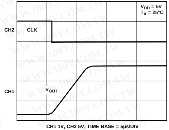
Figure 21. Half-Scale Setting (1/4 to 3/4 Scale Code Change)
