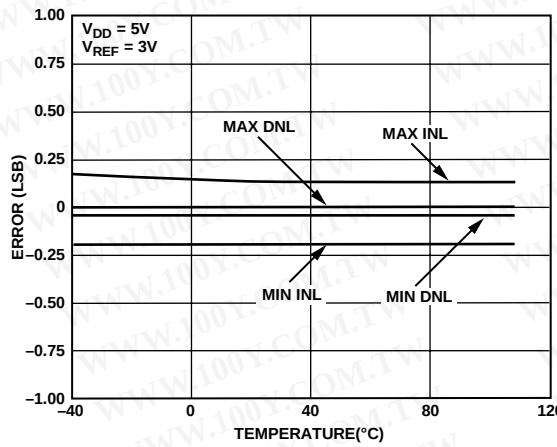
Figure 13. AD5302 INL Error and DNL Error vs. Temperature
