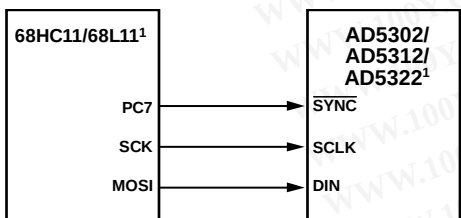
Figure 35. AD5302/AD5312/AD5322 to 68HC11/68L11 Interface
