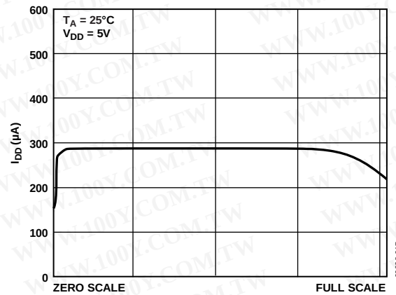
Figure 17. Supply Current vs. Code
