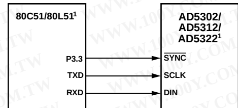
Figure 36. AD5302/AD5312/AD5322 to 80C51/80L51 Interface
