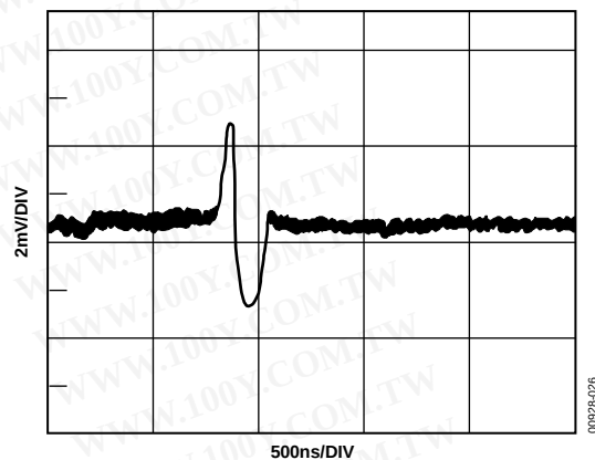
Figure 26. DAC-to-DAC Crosstalk
