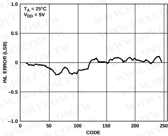
Figure 6. AD5302 Typical INL Plot
