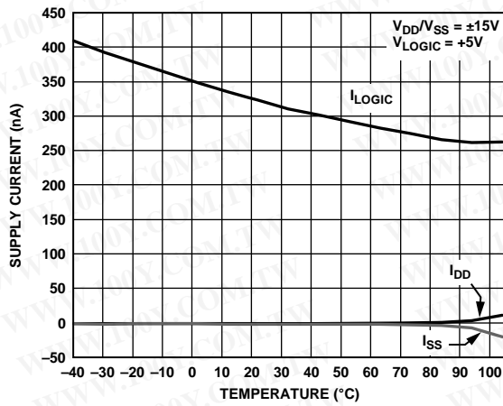
Figure 37. Supply Current ( I_{DD} , I_{SS} , I_{LOGIC} ) vs. Temperature
