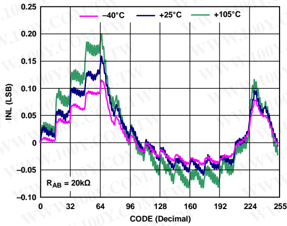
Figure 25. R-INL in Normal Mode vs. Code vs. Temperature (AD5291)
