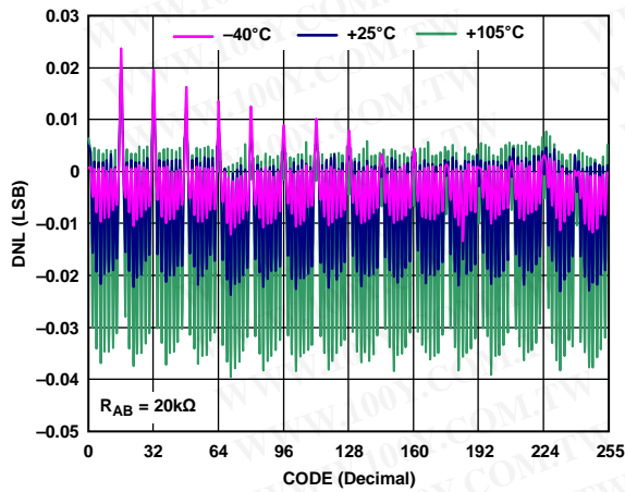
Figure 26. R-DNL in Normal Mode vs. Code vs. Temperature (AD5291)
