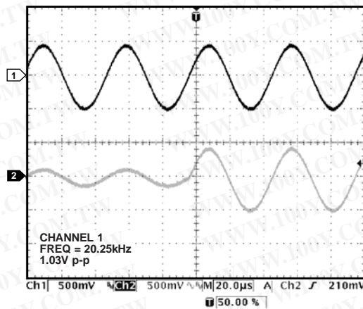
Figure 75. Zipper Noise Detector
