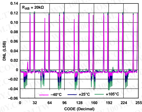
Figure 24. R-DNL in R-Perf Mode vs. Code vs. Temperature (AD5291)
