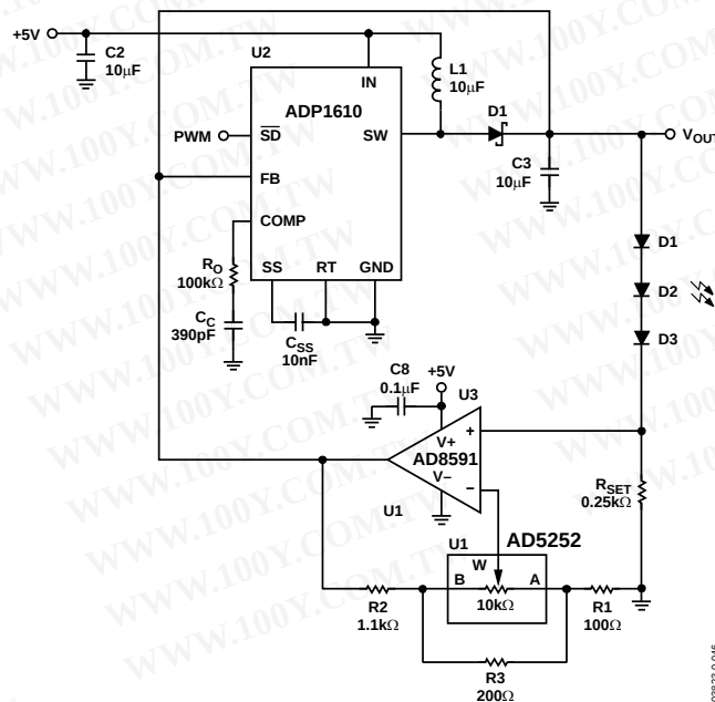
Figure 46. High Power, Adjustable LED Driver
