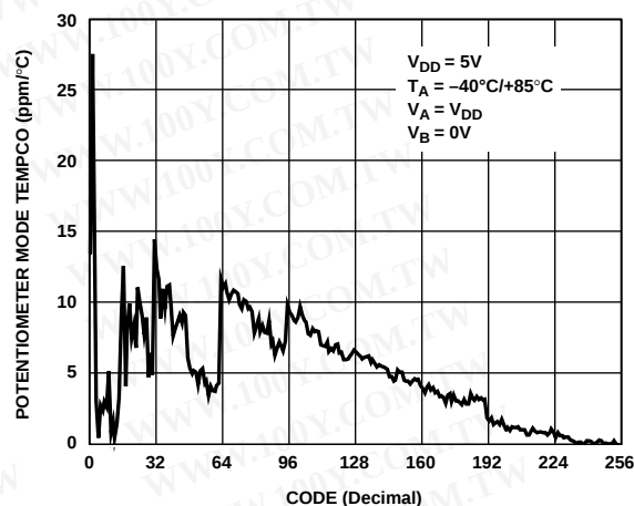
Figure 12. AD5252 Potentiometer Mode Tempco \Delta V_{WB}/\Delta T vs. Code
