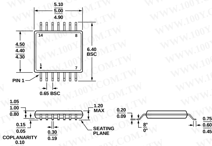
Figure 47. 14-Lead Thin Shrink Small Outline Package [TSSOP] (RU-14)
