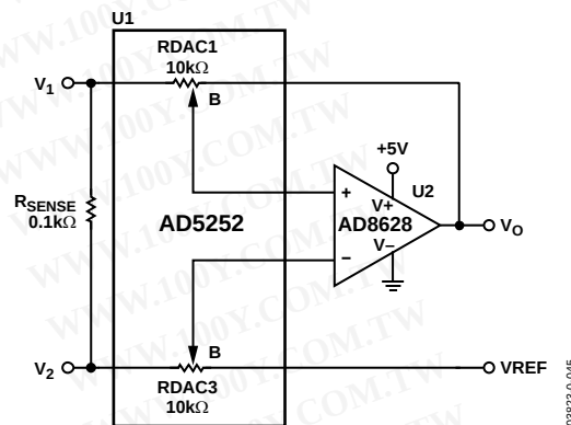
Figure 45. Current-Sensing Amplifier
