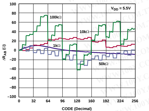
Figure 17. AD5252 \Delta R_{AB} vs. Code, T_A = 25^\circ\text{C}
