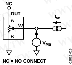
Figure 27. Resistor Position Nonlinearity Error (Rheostat Operation; R-INL, R-DNL)
