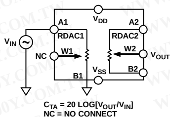
Figure 36. Analog Crosstalk
