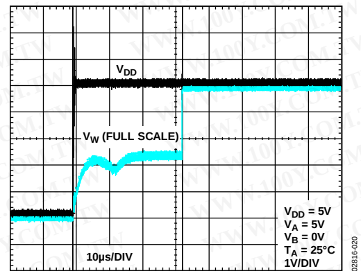
Figure 21. Power-On Reset
