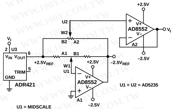
Figure 52. 10-Bit Bipolar DAC
