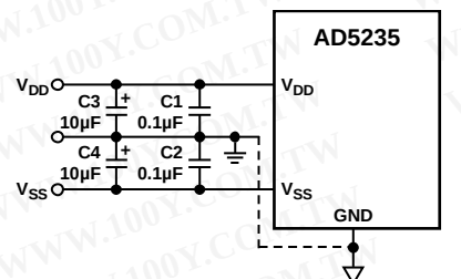
Figure 43. Power Supply Bypassing
