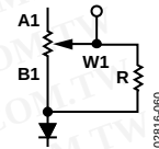
Figure 61. Resistor Scaling with Pseudo Log Adjustment Characteristics
