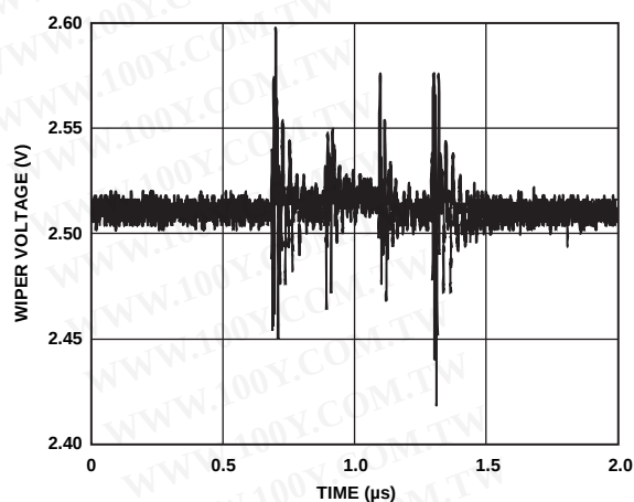
Figure 25. Digital Feedthrough
