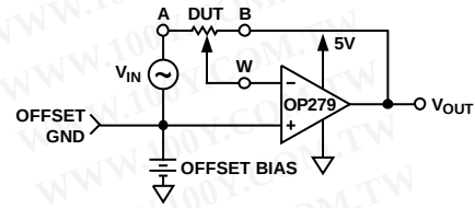
Figure 31. Inverting Gain
