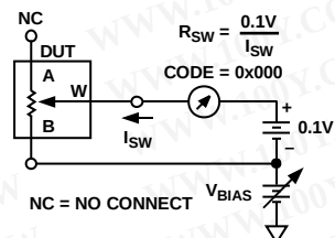
Figure 33. Incremental On Resistance
