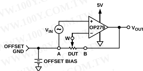
Figure 31. Noninverting Gain
