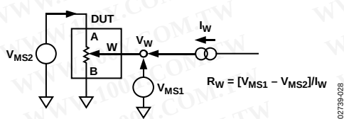
Figure 28. Wiper Resistance
