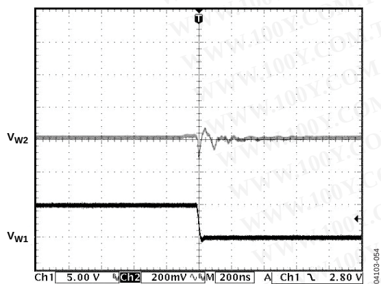
Figure 26. Digital Crosstalk
