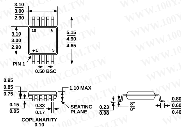
Figure 49. 10-Lead Mini Small Outline Package [MSOP] (RM-10) Dimensions shown in millimeters
